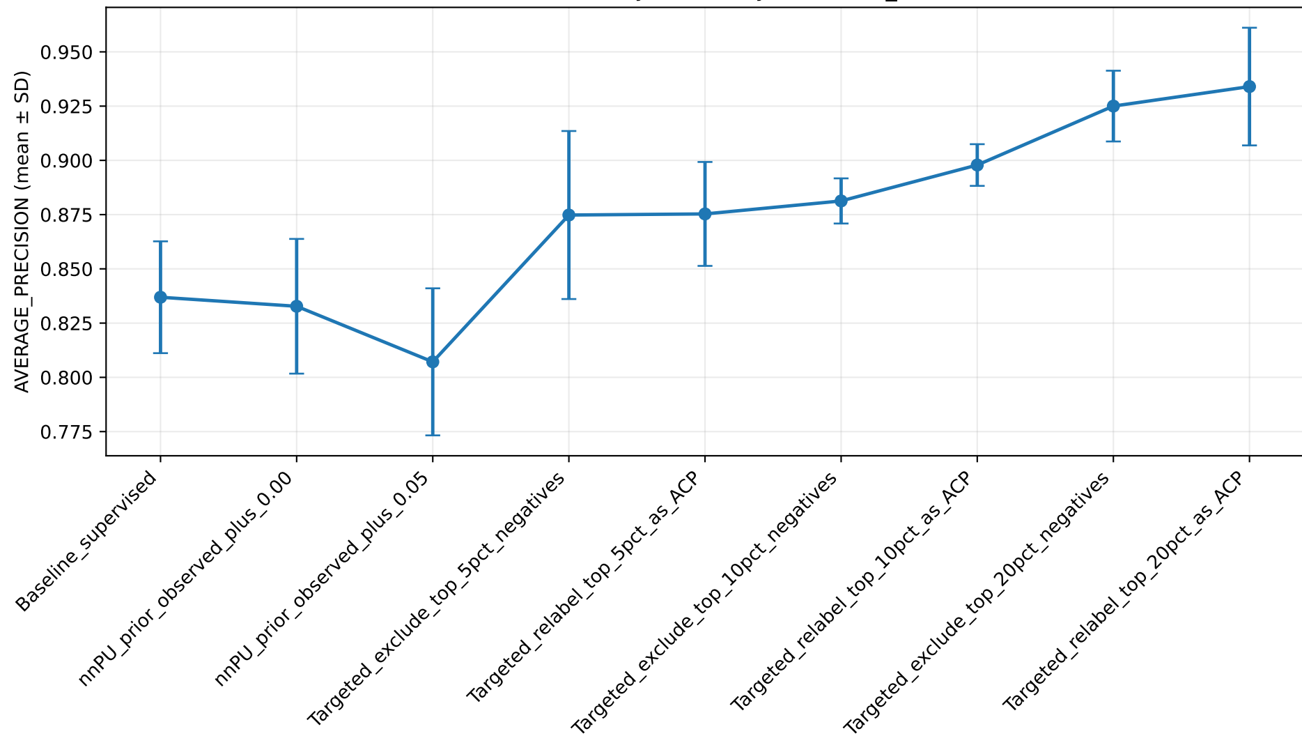
Set 1 label-uncertainty sensitivity: AVERAGE_PRECISION
